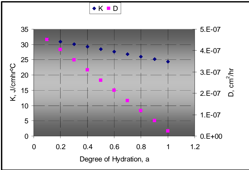
Figure 24 \alpha 's effect on K & D. ( T=20^\circ\text{C} and \text{RH}=0.9 )
